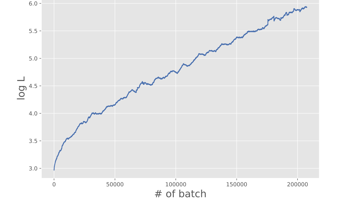
Log of the Lipsitz constant of the gradient per batch
